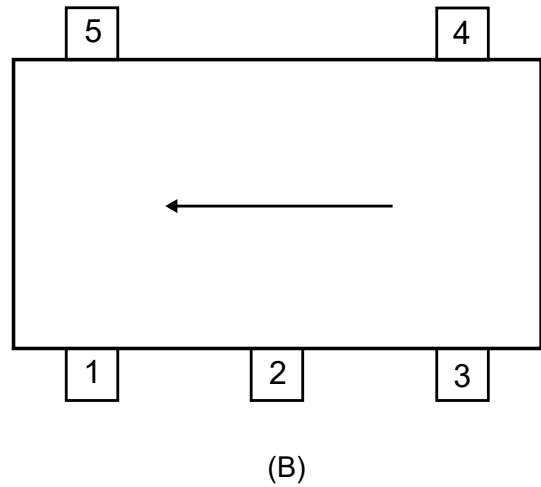
Figure 27: Measuring unipolar current of a busbar placed above the CT220 where (A) shows the direction of the unipolar current and magnetic field, and (B) is the direction of unipolar current flow with respect to the CT220 package.
