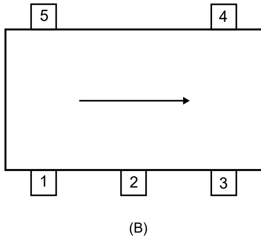
Figure 26: CT220 measuring unipolar current in a busbar below it where (A) indicates the unipolar current and magnetic field directions, and (B) is the direction of unipolar current flow that the CT220 must be oriented.
