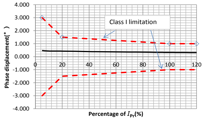
Figure 2: Phase displacement vs. primary current
