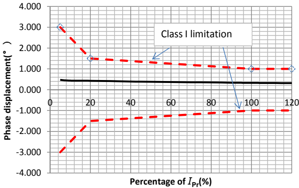
Figure 1: Accuracy vs. primary current
