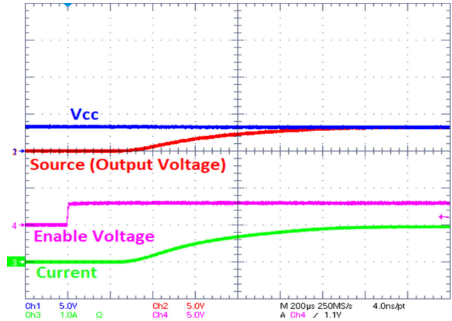
Figure 11. Slew Rate Control for NIS6432
