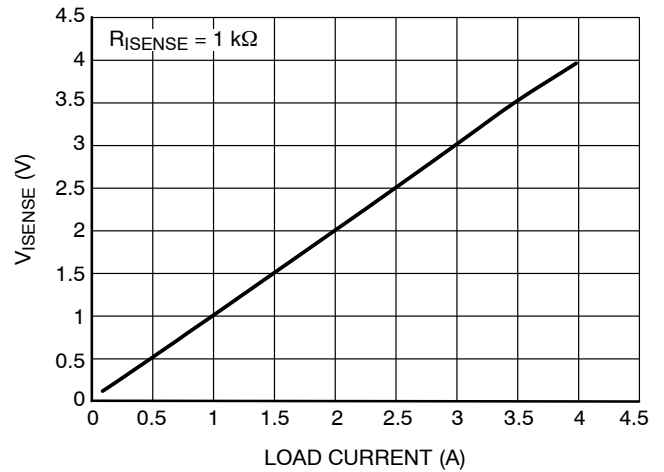
Figure 15. V_{ISENSE} vs Load Current
