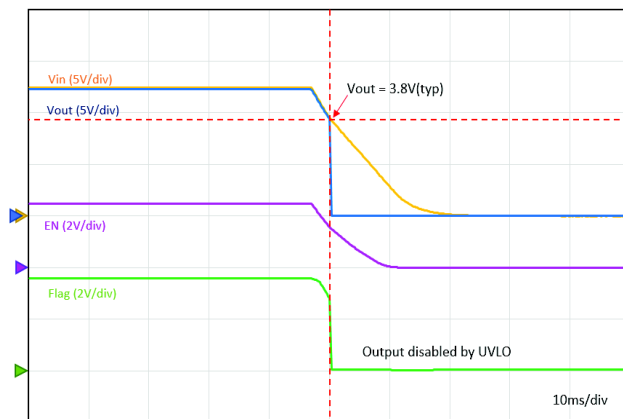
Figure 7. UVLO
