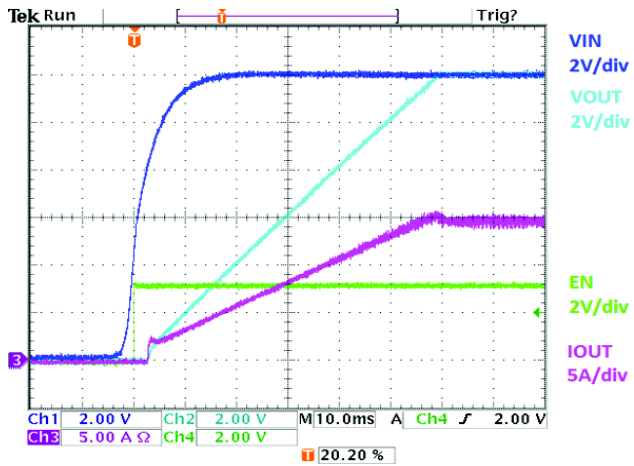
Figure 21. Start Up by VIN ( I_{out} = 15\text{ A} )
