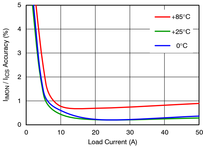
Figure 11. I MON /I CS Accuracy vs. Load Current
