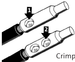
Matrix holder V1320, matrix P13M, punch P13D.
