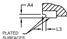
SECTION C-C
