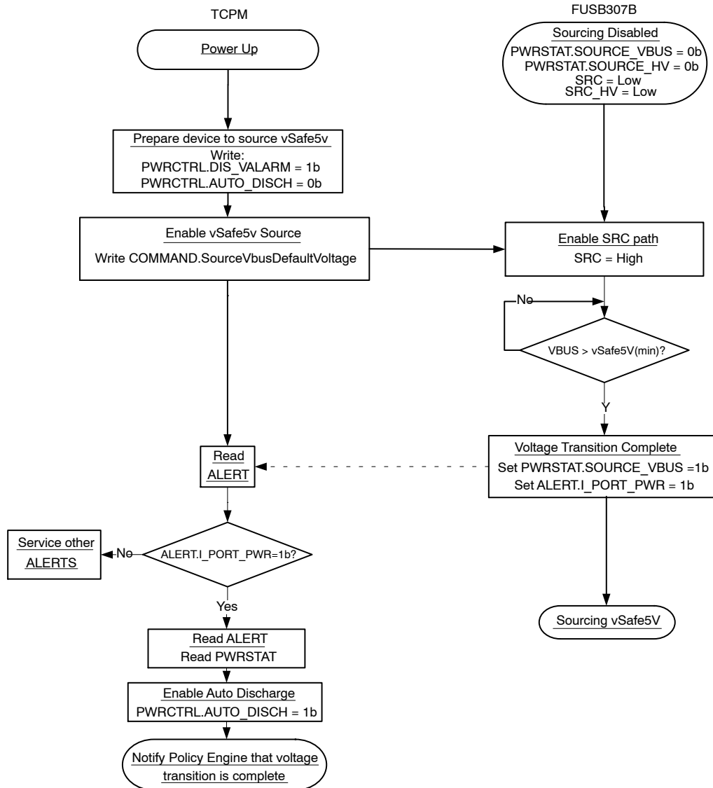
Figure 12. Transition to vSafe5V on Power Up
