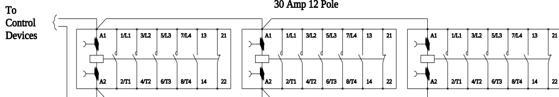
Wiring Diagram Class LE 30 Amp 12 Pole
