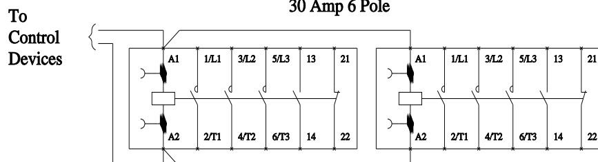
Wiring Diagram Class LE 30 Amp 6 Pole
