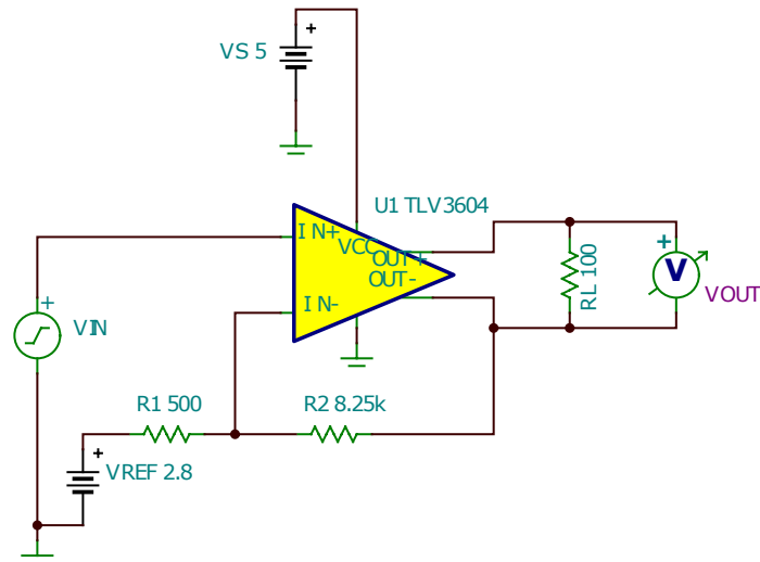
Figure 8-5. Non-Inverting Comparator with Hysteresis Circuit
