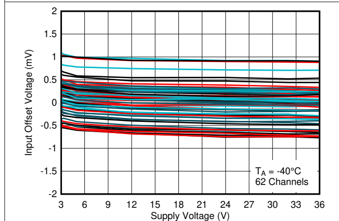
Figure 6-16. Input Offset Voltage vs. Supply Voltage at -40^\circ\text{C}
