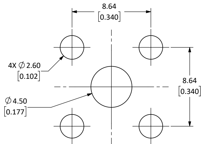
RECOMMENDED MOUNTING HOLES
