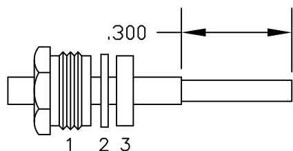
ASSEMBLY (A)
