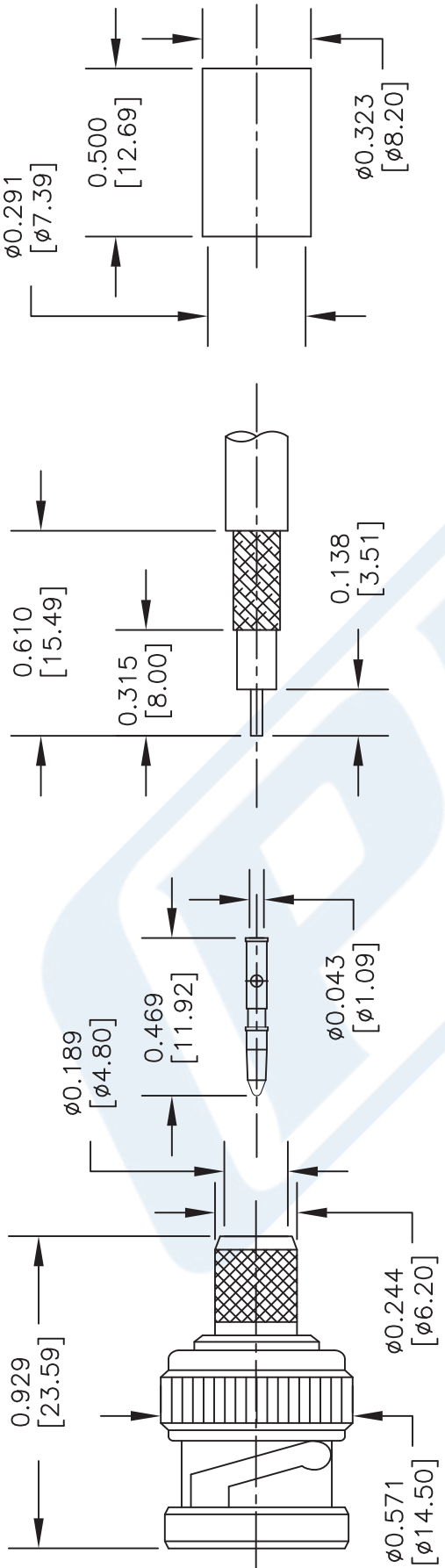
CENTER CONTACT
