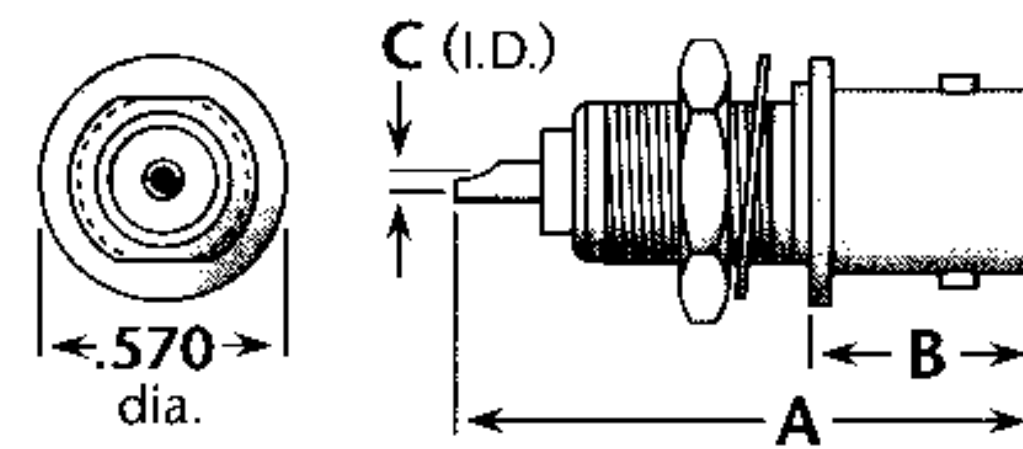
Figure 2 (Front mount, pressurized [non-hermetic], with mounting gasket)
