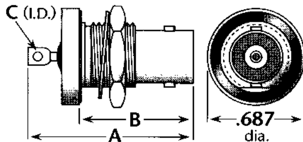
Figure 3 (Rear mount, hermetically sealed, with mounting gasket)
