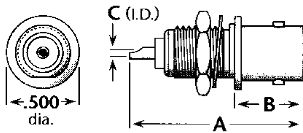
Figure 1 (Front mount)
