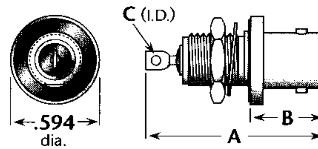
Figure 4 (Front mount, hermetically sealed, with mounting gasket)
