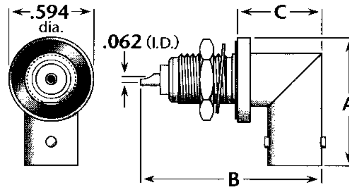
Figure 5 (Right angle, solder pot contact)
