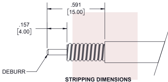
STRIPPING DIMENSIONS
