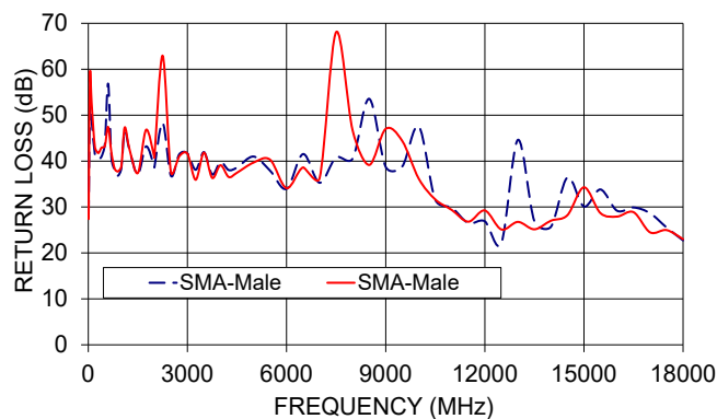
141-8SM+ RETURN LOSS
