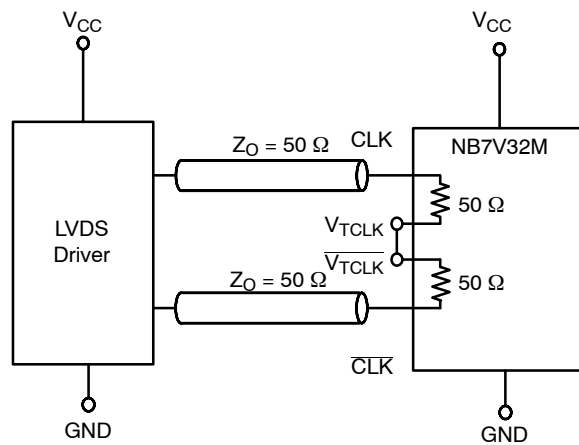
Figure 13. LVDS Interface
