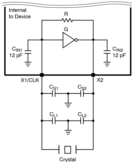
Figure 3. Using a Crystal as Reference Clock
