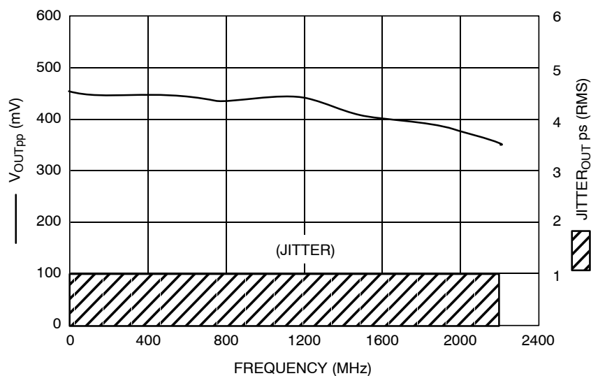
Figure 4. F_{\text{max}} /Jitter
