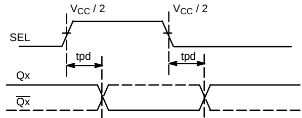
Figure 11. SEL to Qx Timing Diagram
