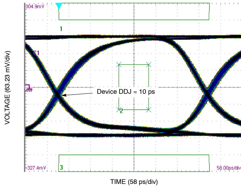
Figure 9. Typical Output Waveform at 2.488 Gb/s with PRBS 2^{23}-1 and OC48 mask (V_{INPP} = 100 \text{ mV}; \text{Input Signal DDJ} = 14 \text{ ps})
