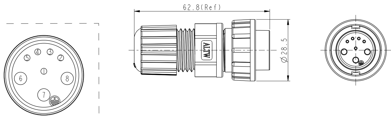
Conn. Pin Assignments Front View
