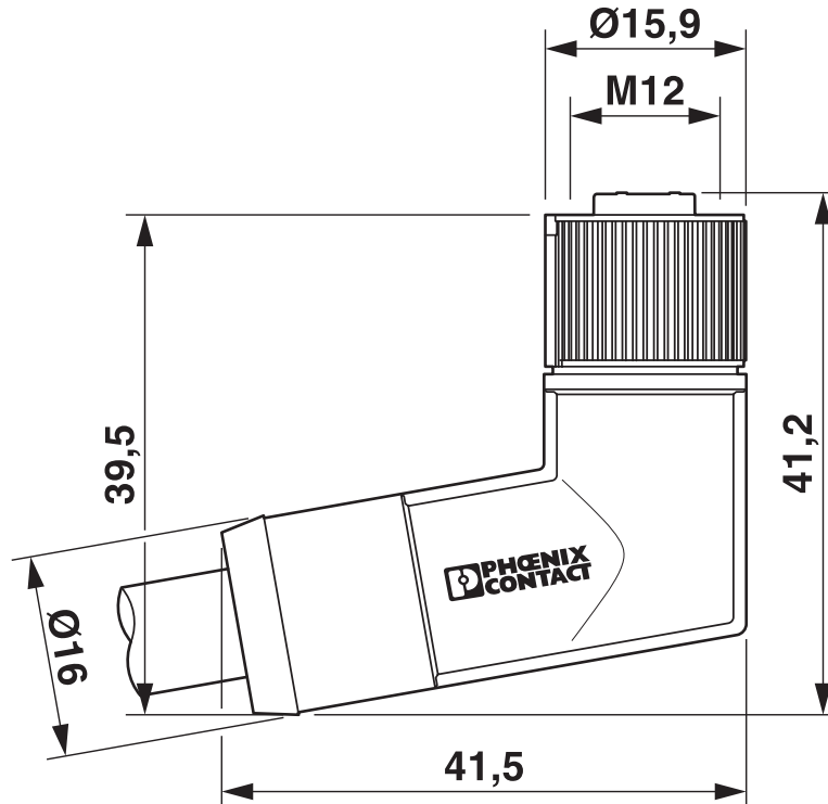
Dimensional drawing
