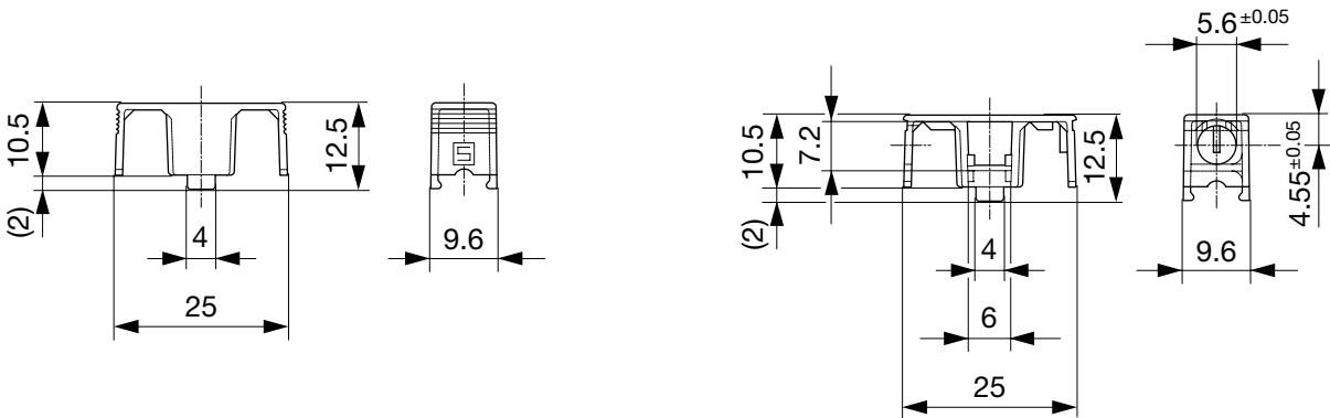
Variants 0853.0551, 0853.0571, 0853.0573 and 0853.0575
