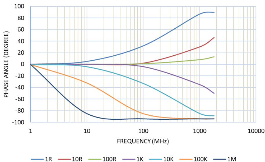
MLF14 FREQUENCY x PHASE ANGLE
