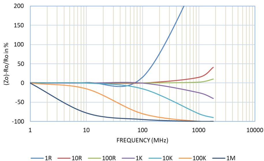
MLF14 FREQUENCY x IMPEDANCE
