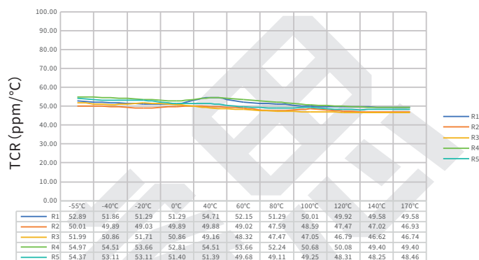
TCR Test Curve -EBWK2512 3mΩ
