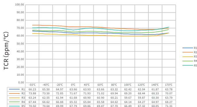
TCR Test Curve -EBWK2512 2mΩ
