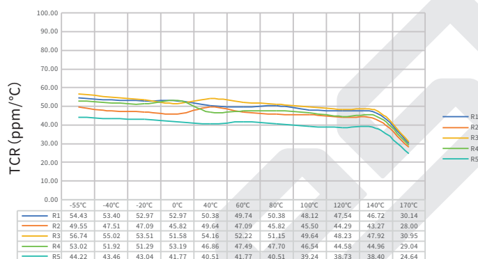
TCR Test Curve -EBWK2512 4mΩ
