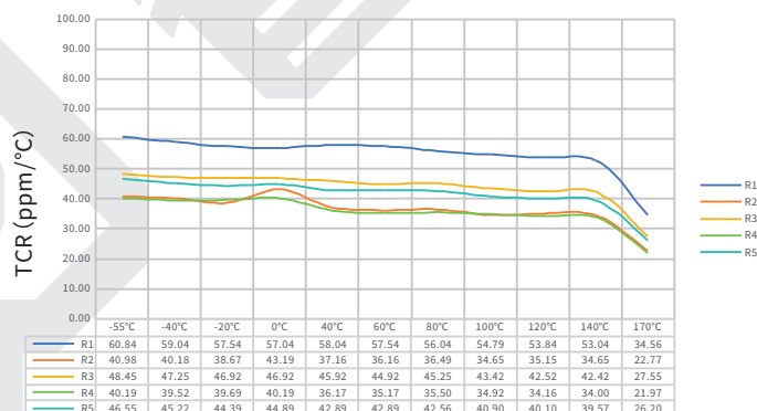
TCR Test Curve -EBWK2512 5mΩ
