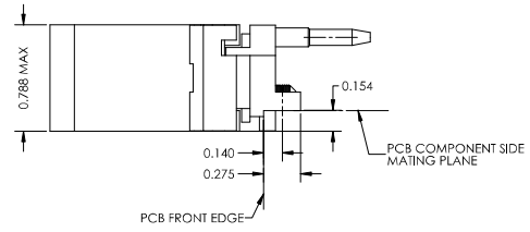
TOP HANDLE DETAIL
