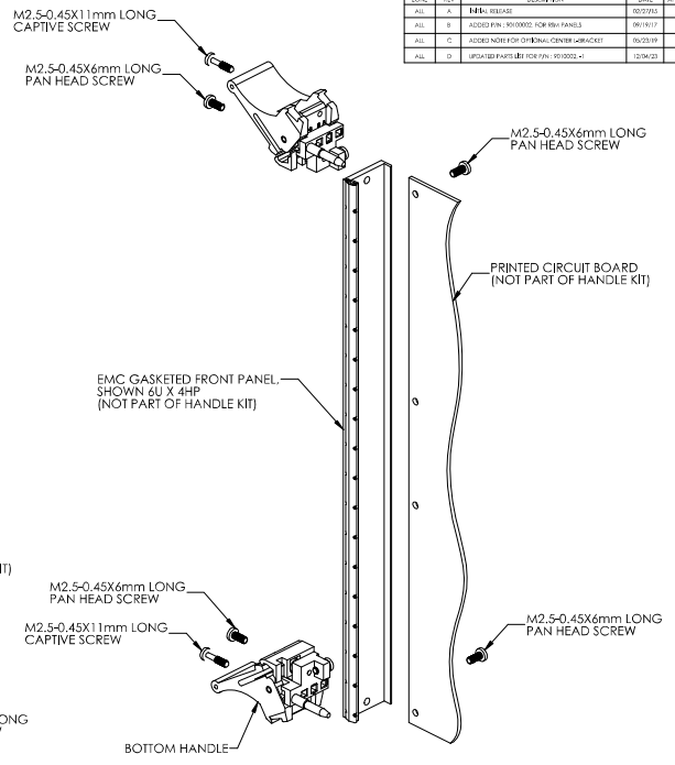
EXPLODED VIEW 6U OR 9U PLUG-IN CARD ASSEMBLY
