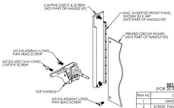
EXPLODED VIEW 3U RTM PLUG-IN CARD ASSEMBLY
