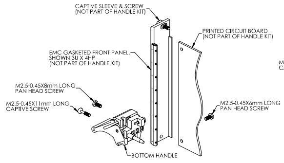
EXPLODED VIEW 3U FRONT PLUG-IN CARD ASSEMBLY
