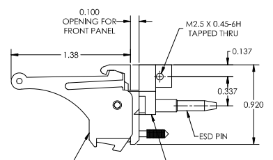
BOTTOM HANDLE DETAIL
