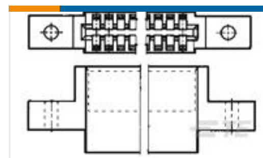
TE Part #1-583718-5 TW LEAF CRP HSG. 40-POS.
