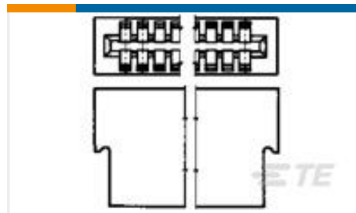
TE Part #1-583717-1 TW-LEAF CRP HSG 25 POS 100 C/L
