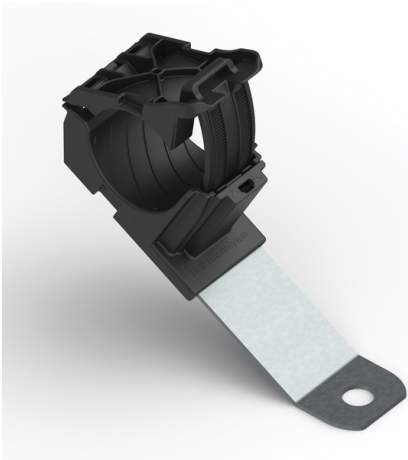
Ratchet P-Clamp, 0.76 - 1.42" Bundle Dia, 30° Long, 0.51" Hole Dia, PA66HIRHSUV/SS304, Black, 140/ctn
