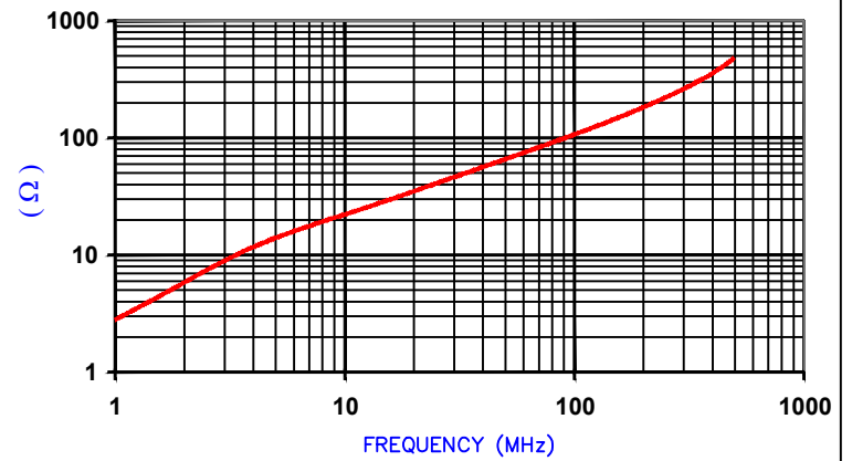
AGILENT E4991A Impedance/Material Analyzer HP 16092A-Test Fixture TEST REF. 4481
