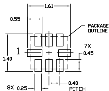
DETAIL A ALTERNATE CONSTRUCTIONS
