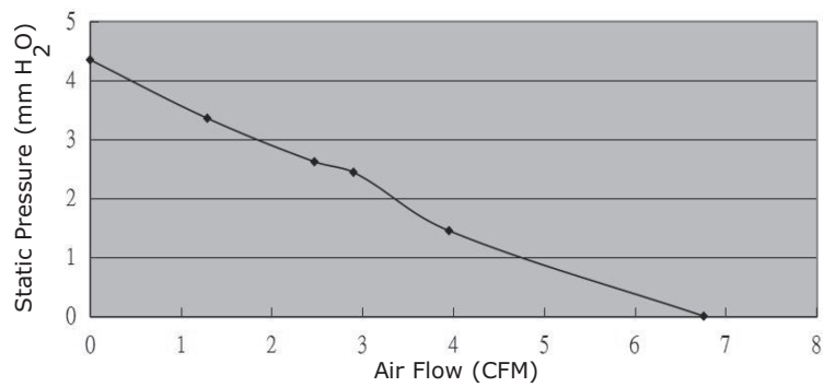
CFM-4010C-280-296
