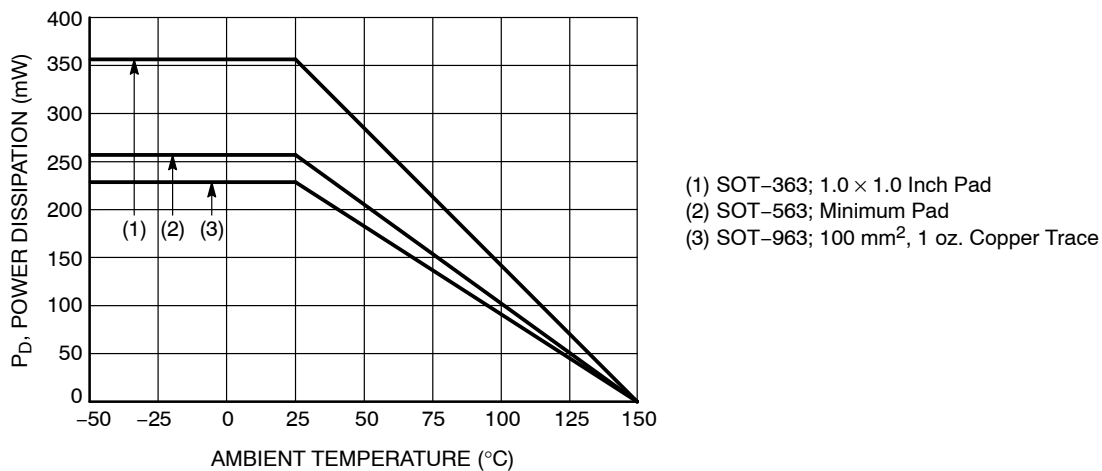
Figure 1. Derating Curve
