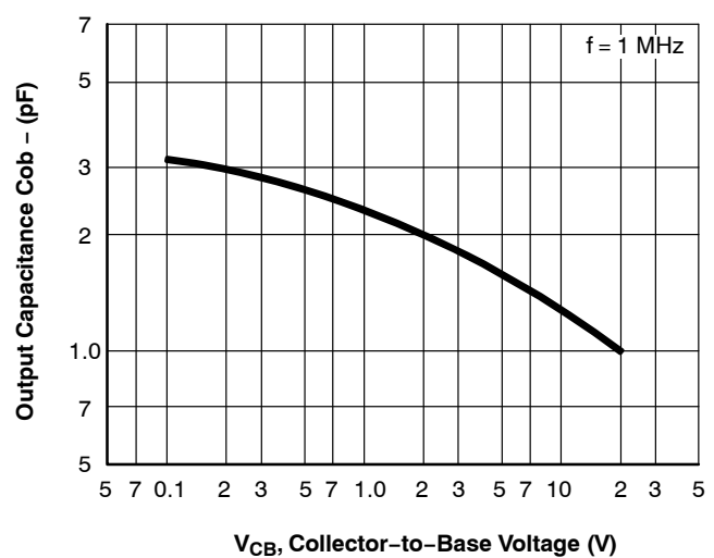
Figure 4. C_{ob} - V_{CB}
