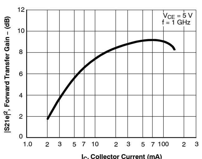
Figure 6. |S_{21e}|^2 - I_C
