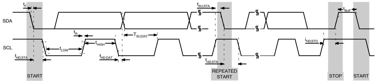
Figure 4. I²C Interface Timing for Fast and Slow Modes
