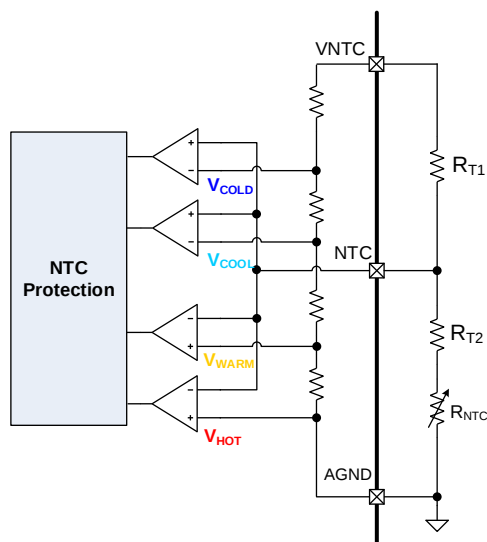
Figure 6: NTC Protection Circuit
