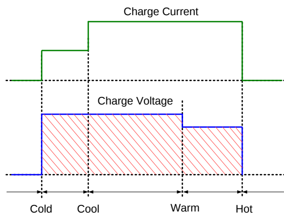
Figure 7: NTC Window
