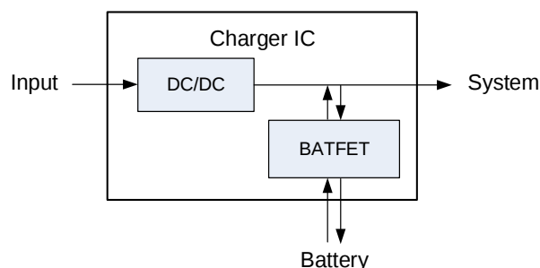
Figure 3: NVDC Power Path Management Structure
