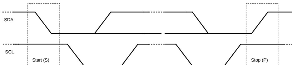
Figure 11: Start and Stop Conditions
