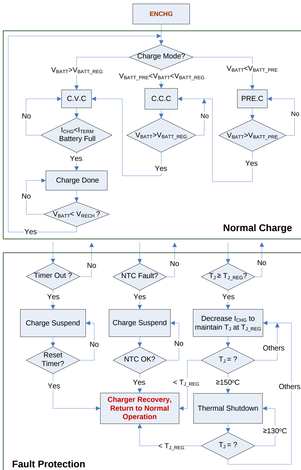
Figure 19: Charging Process
