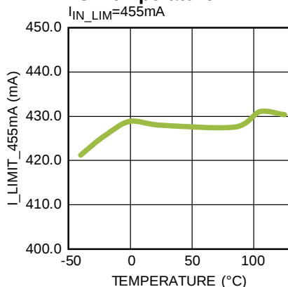
I_Limit_455mA vs. Temperature I_{IN\_LIM}=455mA
