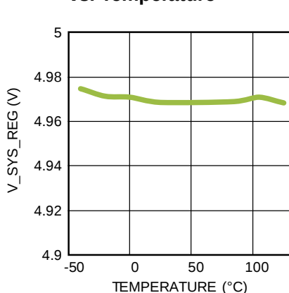
System Regulation Voltage vs. Temperature
