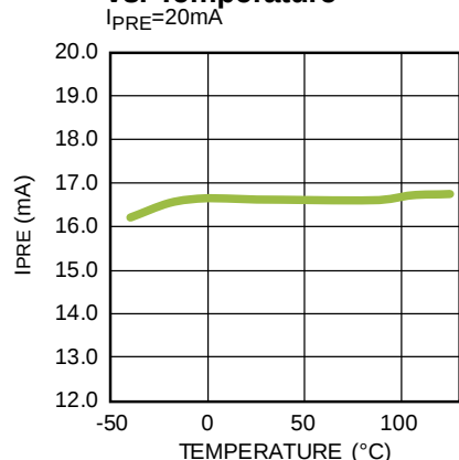
Pre-Charge Current vs. Temperature I_{PRE}=20mA
