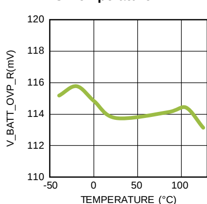
Battery OVP Voltage vs. Temperature
