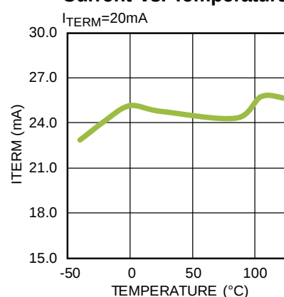
Battery Termination Current vs. Temperature I_{TERM}=20mA
