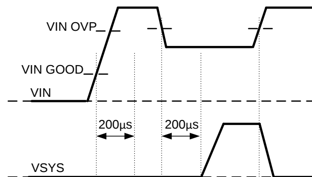
Figure 3: Input Power Detection Operation
