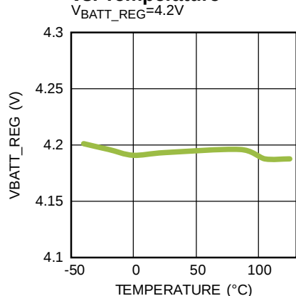
Battery Regulation Voltage vs. Temperature V_{BATT\_REG}=4.2V
