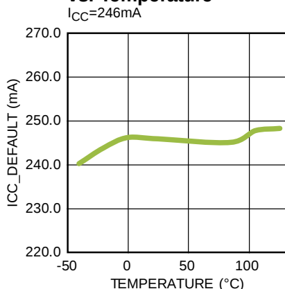
Fast Charge Current vs. Temperature I_{CC}=246mA
