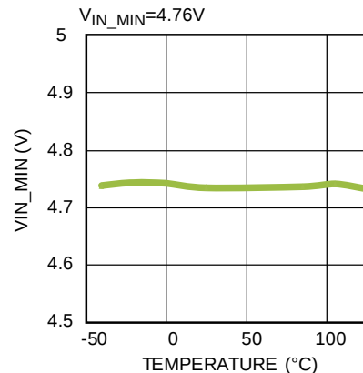
Input Regulation Voltage vs. Temperature V_{IN\_MIN}=4.76V
