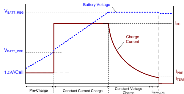
Figure 2: Battery Charging Cycle
