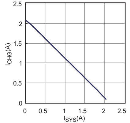
Current Sharing
