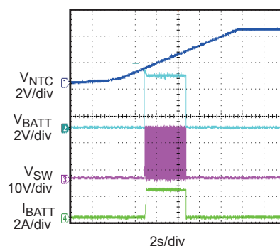
NTC Control
