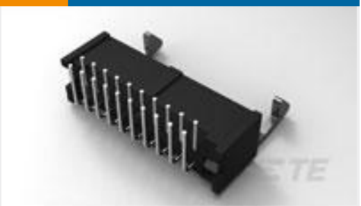
TE Part # 3-1761607-3 IDC LOW PRO HDR 40P RA LG LAT
