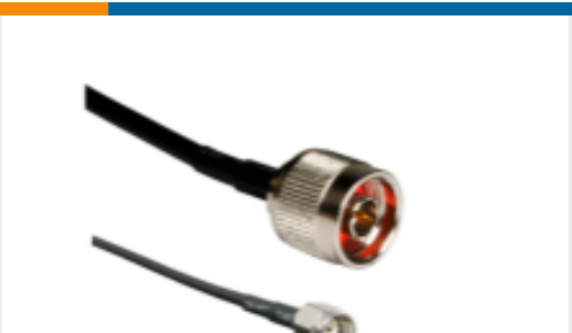
TE Part #C58LL-RPSM-2438-NM RP-SMA to N Type 2458mm RG58
