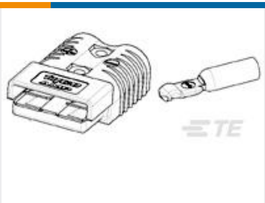
TE Part #1604042-3 KIT, 175A, 1/0 AWG, RED
