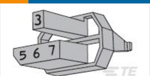
TE Part #5-100526-6 Z-PACK F.CODING KEY
