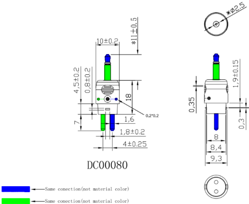
T-PLUG Male Mono 2.5mm x 11mm
