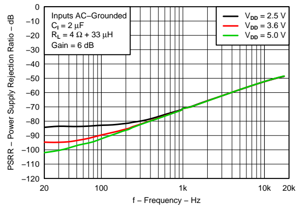
Figure 22. Power Supply Rejection Ratio vs Frequency
