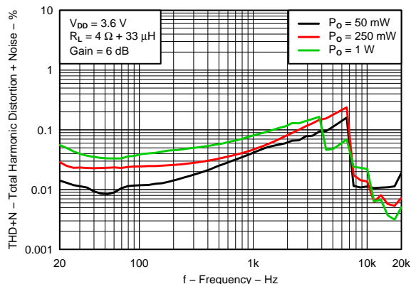
Figure 18. THD + Noise vs Frequency
