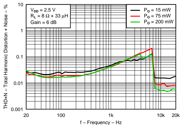
Figure 16. THD + Noise vs Frequency
