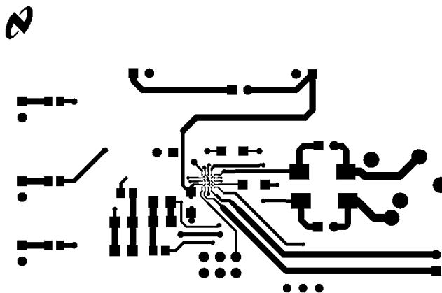
Figure 74. Top Layer
